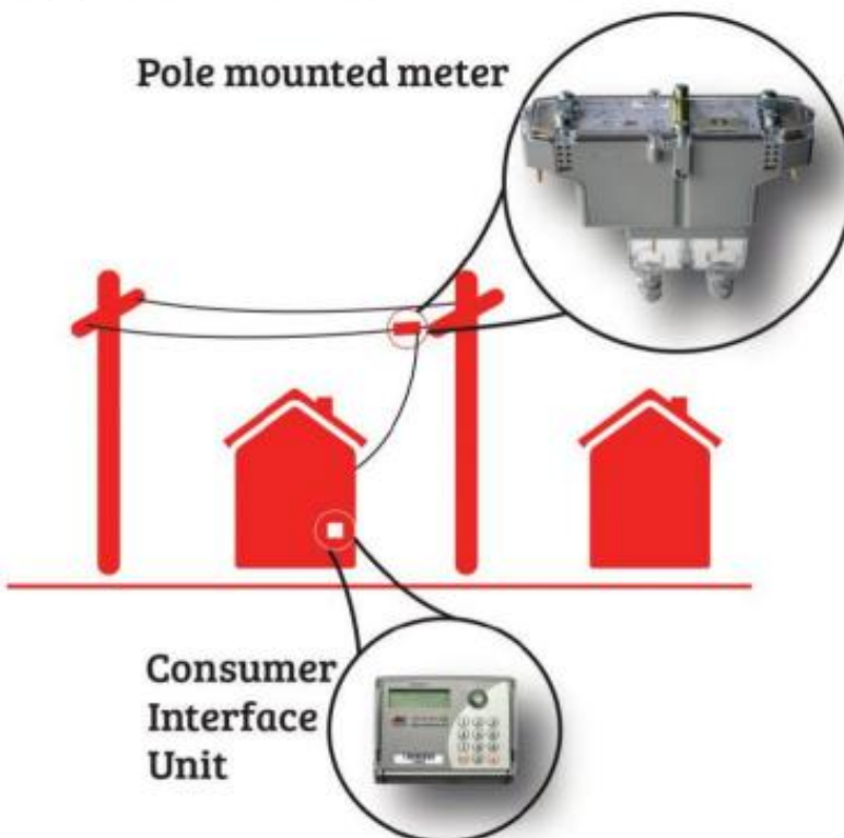
Figure 1: Installation scheme of pole mounted meter and consumer interface unit (CIU)
